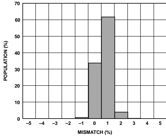
Figure 11. Self-Test Mismatch at 25°C ( V_{RATIO} = 5 V )
