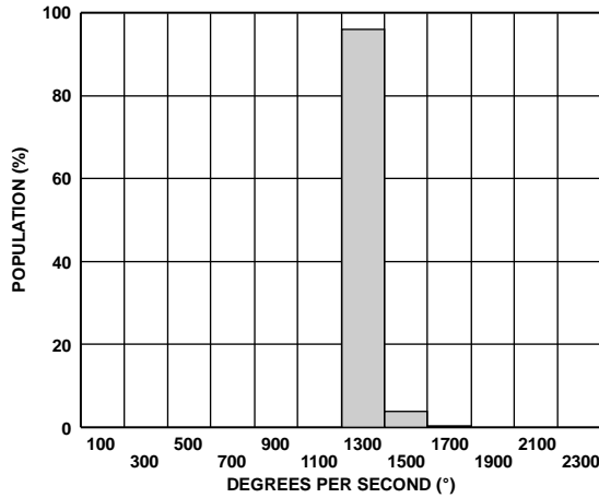
Figure 10. ST2 Output Change at 25°C ( V_{RATIO} = 5 V )
