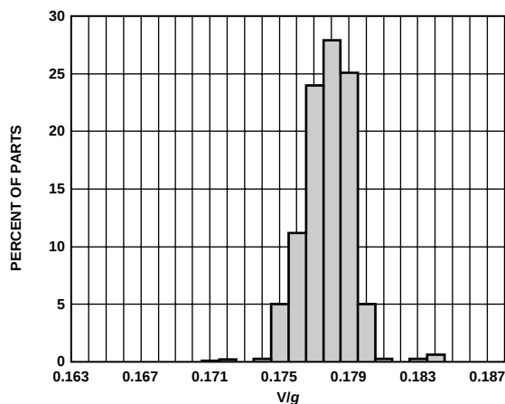
Figure 5. X-Axis Output Sensitivity Distribution at X_{OUT}
