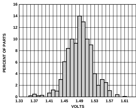
Figure 3. X-Axis 0 g BIAS Output Distribution
