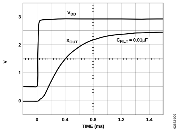
Figure 10. Typical Turn-On Time
