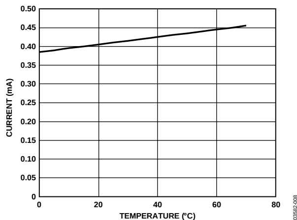
Figure 9. Typical Supply Current vs. Temperature
