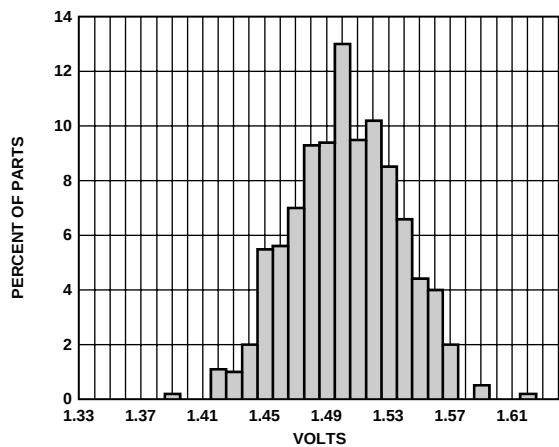
Figure 4. Y-Axis 0 g BIAS Output Distribution
