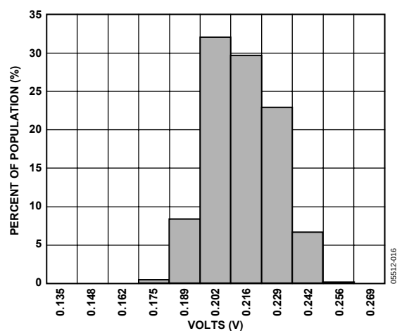
Figure 17. X-Axis Self-Test Response at 25°C
