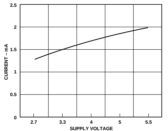
Figure 6. Typical Supply Current vs. Supply Voltage
