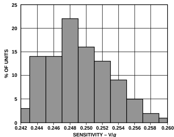
Figure 5. Sensitivity Distribution*
