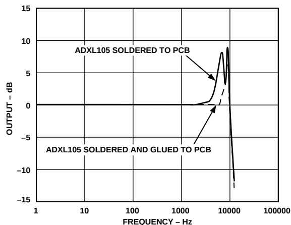
Figure 12. Frequency Response
