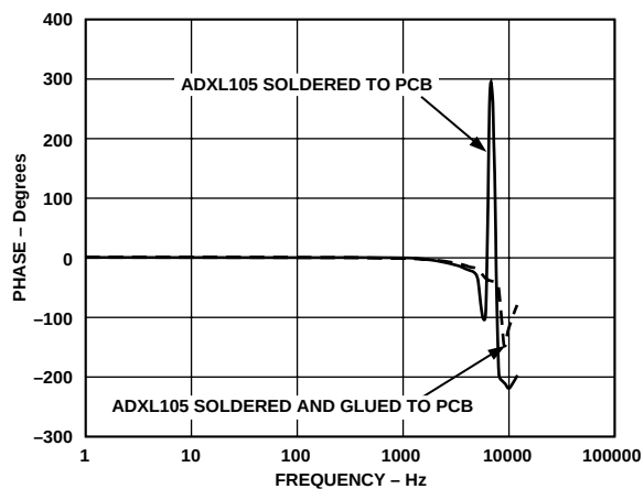
Figure 13. Phase Response
