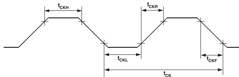
Figure 69. XTAL1 Input
