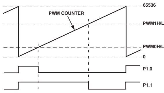
Figure 29. PWM Mode 3
