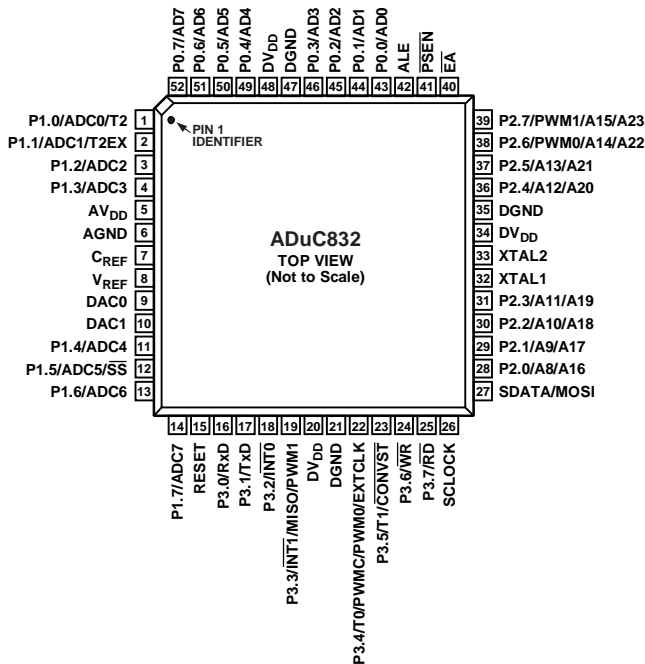
Figure 14. 52-Lead MQFP
