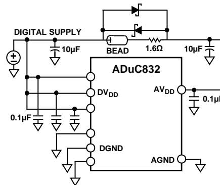
Figure 91. External Single-Supply Connections
