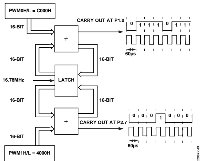
Figure 60. PWM Mode 4
