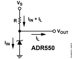
Figure 19. Shunt Reference
