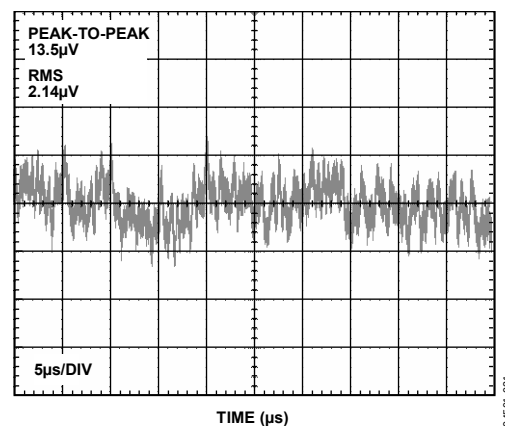
Figure 12. ADR520 Voltage Noise 0.1 Hz to 10 Hz
