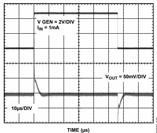
Figure 13. ADR525 Load Transient Response
