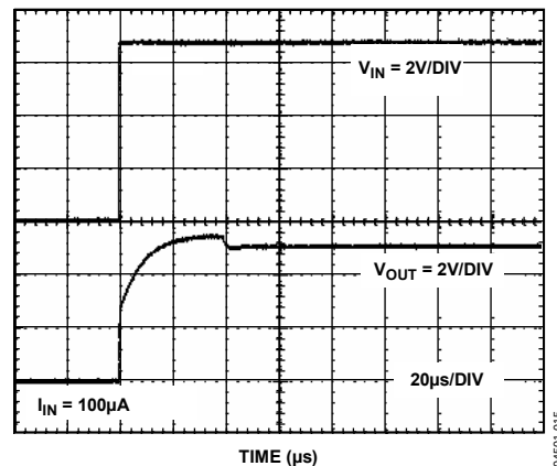
Figure 11. ADR550 Turn-On Response
