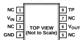
Figure 1. 8-Lead SOIC
