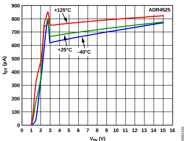
Figure 25. ADR4525 Supply Current vs. Supply Voltage
