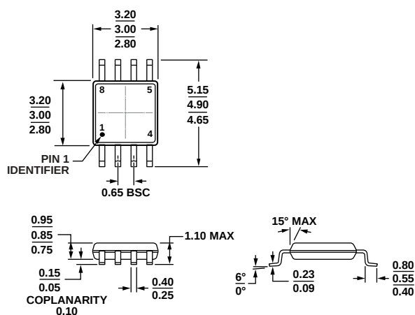
Figure 43. 8-Lead Mini Small Outline Package [MSOP] (RM-8) Dimensions show in millimeters
