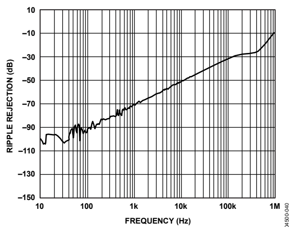
Figure 28. Ripple Rejection
