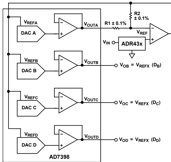
Figure 41. Programmable DAC Reference
