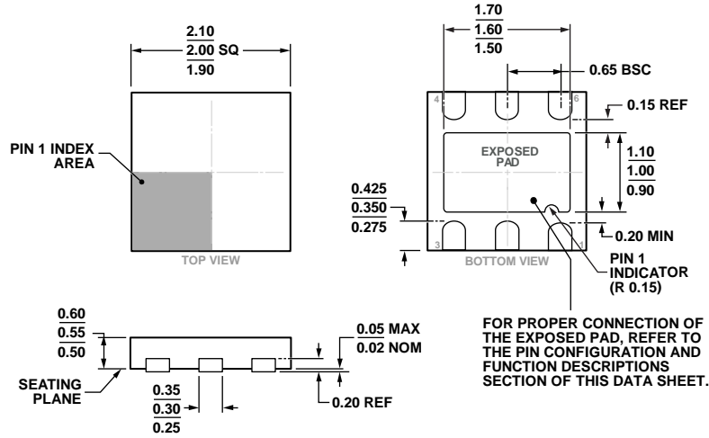
Figure 67. 6-Lead Lead Frame Chip Scale Package [LFCSP_UD] 2.00 mm x 2.00 mm Body, Ultra Thin, Dual Lead (CP-6-3) Dimensions shown in millimeters
