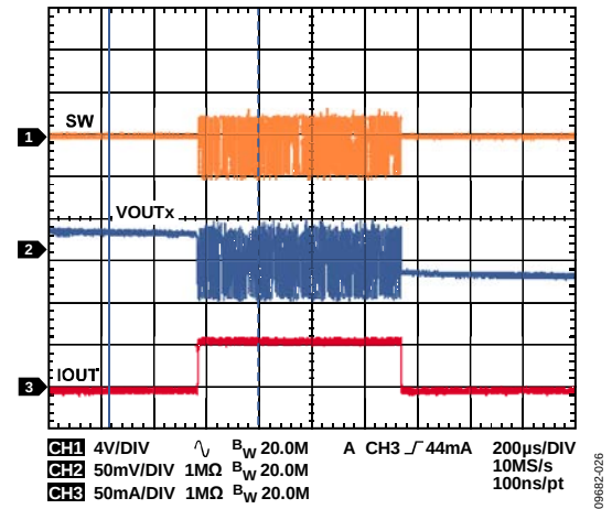
Figure 25. Buck Response to Load Transient, I_{OUT1} from 1\text{ mA} to 50\text{ mA} , V_{OUT1} = 3.3\text{ V} , Auto Mode
