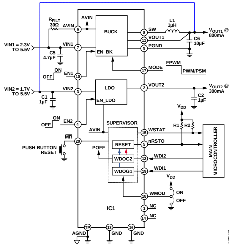
Figure 56. Application Diagram
