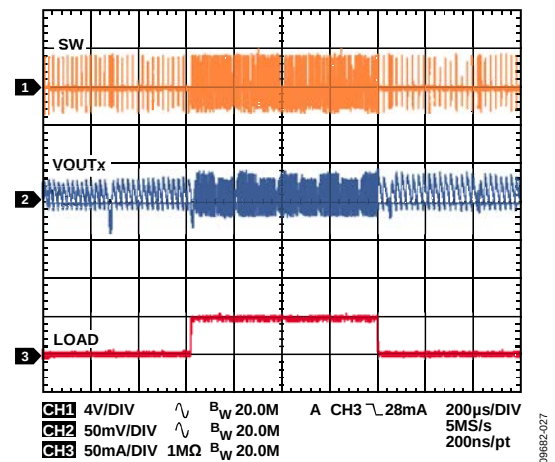
Figure 26. Buck Response to Load Transient, I_{OUT2} from 1\text{ mA} to 50\text{ mA} , V_{OUT1} = 1.8\text{ V} , Auto Mode
