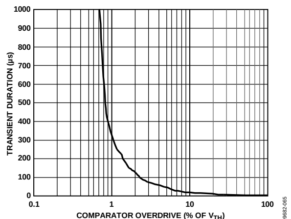
Figure 52. Maximum V_{TH} Transient Duration vs. Reset Threshold Overdrive
