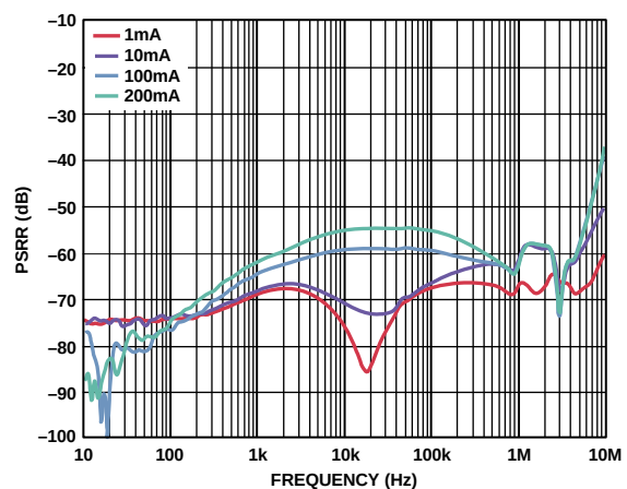
Figure 42. LDO PSRR vs. Frequency, V_{IN2} = 5\text{ V} , V_{OUT2} = 3.3\text{ V}
