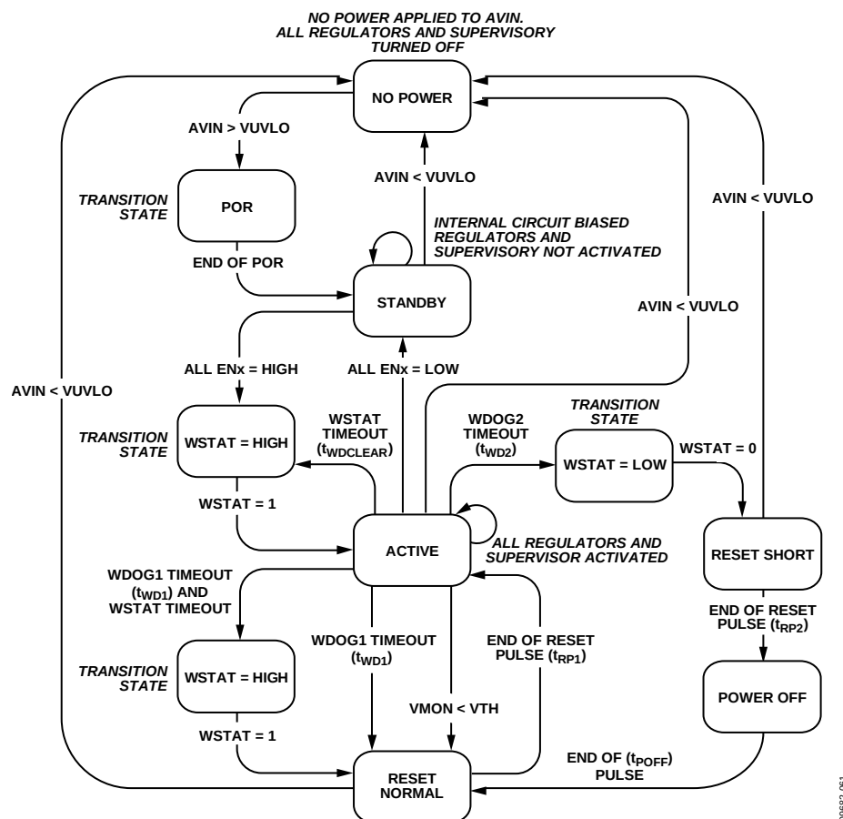
Figure 47. ADP5043 State Flow
