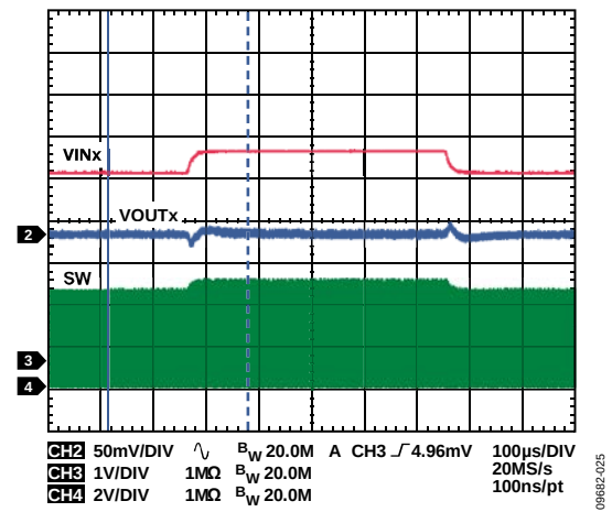
Figure 24. Buck Response to Line Transient, V_{IN} = 4.5\text{ V} to 5.0\text{ V} , V_{OUT1} = 1.8\text{ V} , PWM Mode
