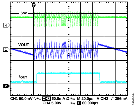
Figure 26. BUCK1 Response to Load Transient, I_{OUT1} from 1 mA to 50 mA, V_{OUT1} = 3.3\text{ V} , Auto Mode
