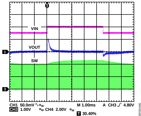
Figure 24. BUCK1 Response to Line Transient, Input Voltage from 4.5 V to 5.0 V, V_{OUT1} = 3.3\text{ V} , PWM Mode
