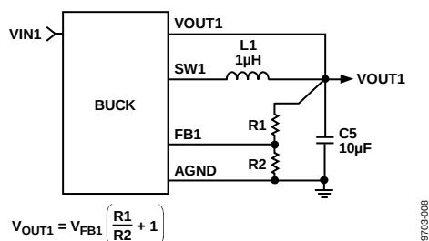
Figure 48. BUCK1 External Output Voltage Setting
