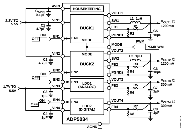
Figure 51. Processor System Power Management with PSM/PWM Control
