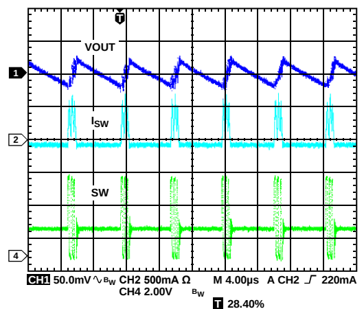
Figure 21. Typical Waveforms, V_{OUT2} = 1.8\text{ V} , I_{OUT2} = 30\text{ mA} , Auto Mode
