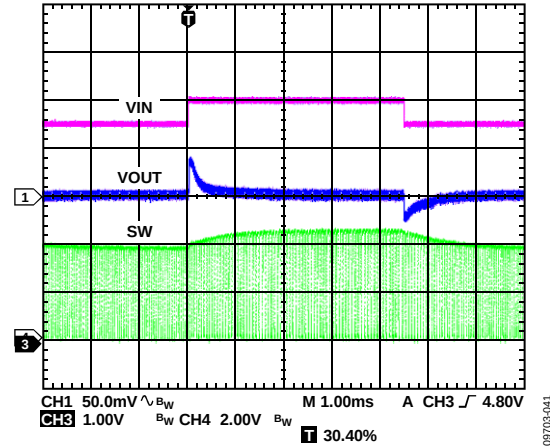
Figure 25. BUCK2 Response to Line Transient, V_{IN2} = 4.5\text{ V} to 5.0 V, V_{OUT2} = 1.8\text{ V} , PWM Mode
