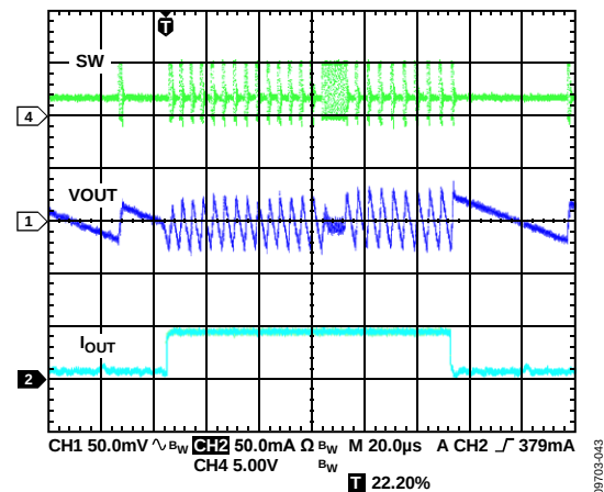
Figure 27. BUCK2 Response to Load Transient, I_{OUT2} from 1 mA to 50 mA, V_{OUT2} = 1.8\text{ V} , Auto Mode
