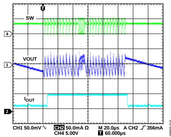
Figure 25. BUCK1 Response to Load Transient, I_{OUT1} = 1\text{ mA} to 50\text{ mA} , V_{OUT1} = 3.3\text{ V} , Auto Mode
