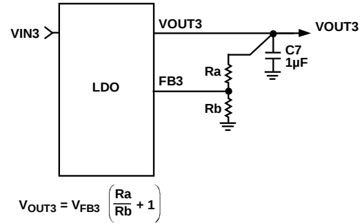
Figure 48. LDO External Output Voltage Setting
