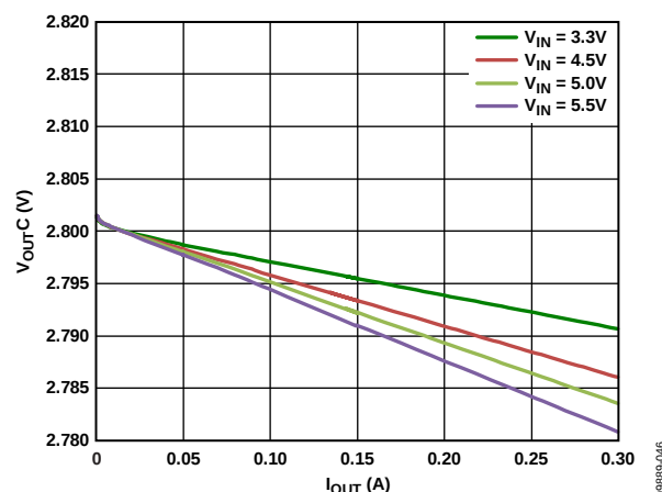
Figure 31. LDO Load Regulation Across Input Voltage, V_{OUT3} = 2.8 \text{ V}
