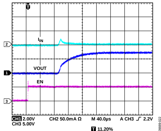
Figure 30. LDO Startup, V_{OUT3} = 3.0 \text{ V} , I_{OUT3} = 5 \text{ mA}
