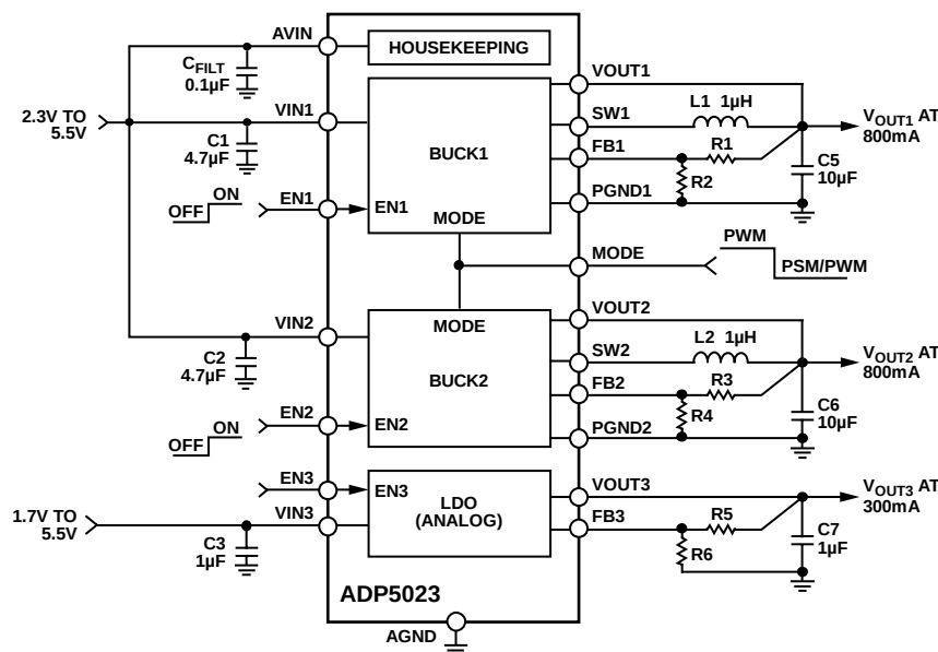
Figure 50. Processor System Power Management with PSM/PWM Control
