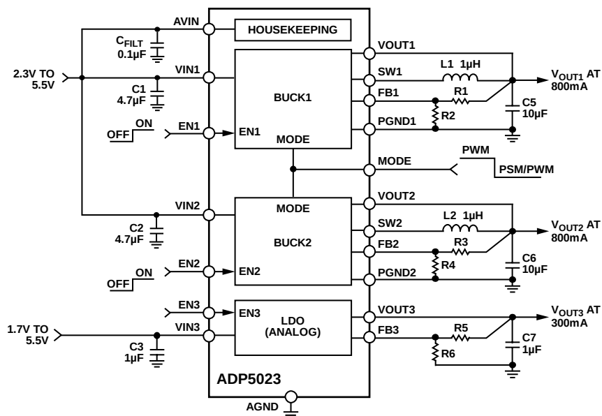
Figure 53. ADP5023 Adjustable Output Voltages with Enable Pins
