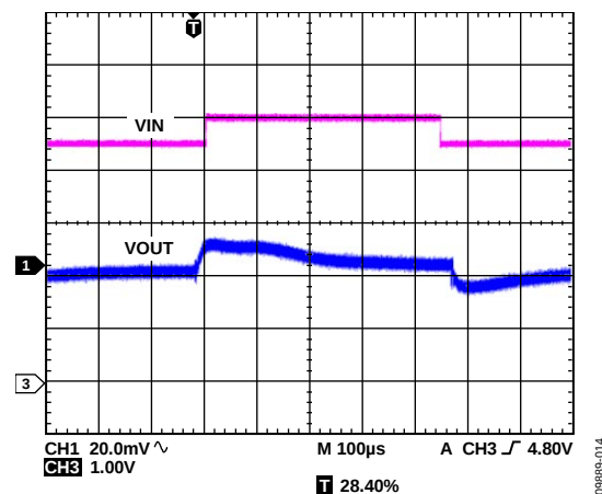
Figure 38. LDO Response to Line Transient, V_{IN} = 4.5\text{ V} to 5.5\text{ V} , V_{OUT3} = 2.8\text{ V}
