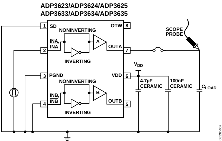
Figure 20. Test Circuit
