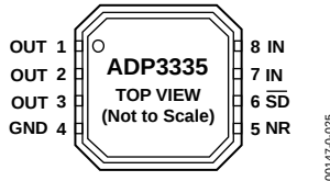
Figure 3. 8-Lead MSOP
