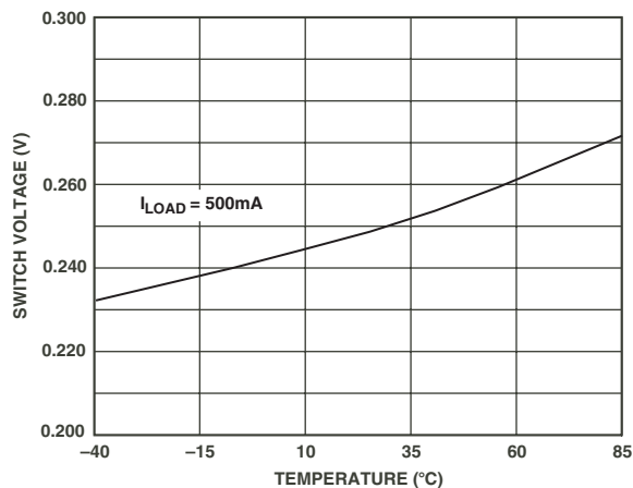
TPC 11. Switch-Sense Resistor Voltage vs. Temperature
