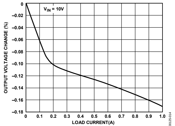
Figure 14. Load Regulation
