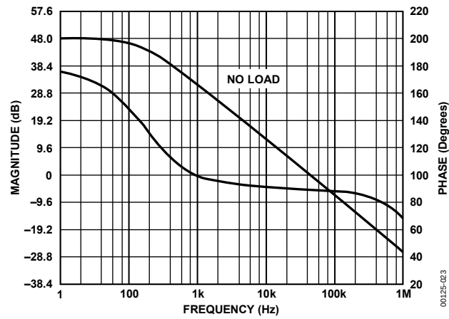
Figure 23. Error Amplifier Gain
