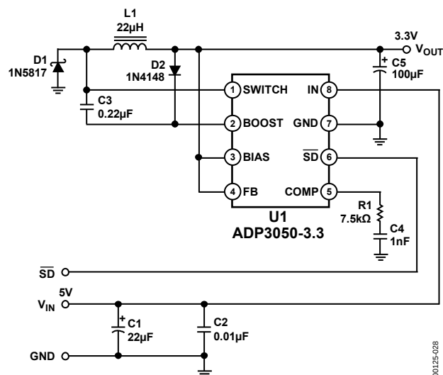
Figure 28. 5 V to 3.3 V Buck Regulator
