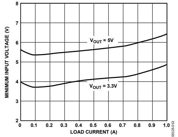
Figure 13. Minimum Input Voltage vs. Load Current
