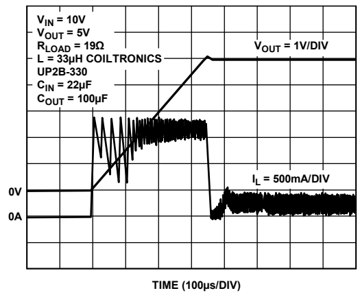
Figure 21. Start-Up from Shutdown
