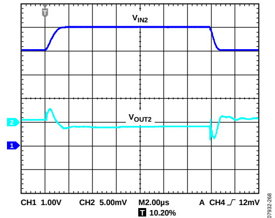
Figure 68. Line Transient Response, V_{OUT2} = 3.3\text{ V} , Load Current = 300 mA, V_{IN2} = 4\text{ V} to 5 V, 1 \mu\text{s} Rise Time
