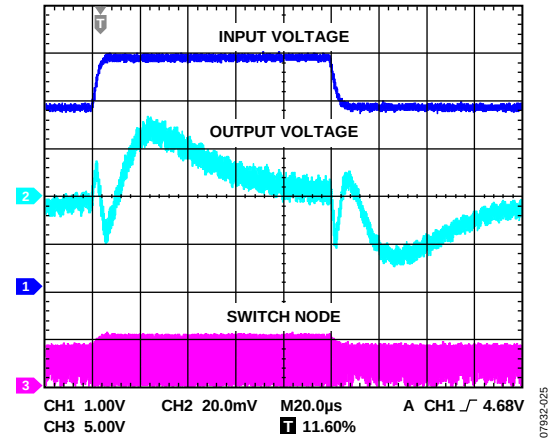
Figure 25. Line Transient, V_{OUT} = 3.3\text{ V} , PWM Mode, 600\text{ mA} , V_{IN1} = 4\text{ V} to 5\text{ V} , 4\text{ }\mu\text{s} Rise Time
