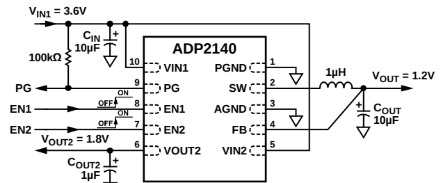
Figure 1. ADP2140 with LDO Connected to V_{IN1}
