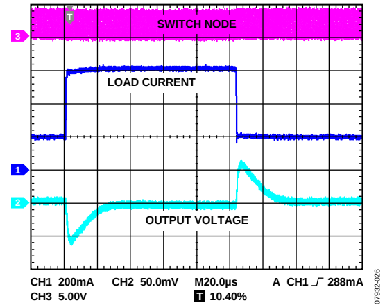
Figure 26. Load Transient, V_{OUT} = 1.8\text{ V} , 200\text{ mA} to 600\text{ mA} , Load Current Rise Time = 200\text{ ns}
