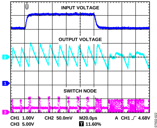
Figure 22. Line Transient, V_{OUT} = 1.2\text{ V} , PSM Mode, 50\text{ mA} , V_{IN1} = 4\text{ V} to 5\text{ V} , 4\text{ }\mu\text{s} Rise Time
