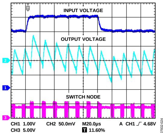
Figure 24. Line Transient, V_{OUT} = 3.3\text{ V} , PSM Mode, 50\text{ mA} , V_{IN1} = 4\text{ V} to 5\text{ V} , 4\text{ }\mu\text{s} Rise Time
