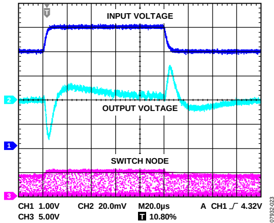
Figure 23. Line Transient, V_{OUT} = 1.2\text{ V} , PWM Mode, 600\text{ mA} , V_{IN1} = 4\text{ V} to 5\text{ V} , 4\text{ }\mu\text{s} Rise Time
