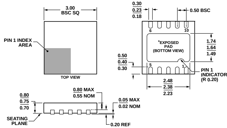
Figure 98. 10-Lead Lead Frame Chip Scale Package [LFCSP_WD] 3 mm × 3 mm Body, Very Very Thin, Dual Lead (CP-10-9) Dimensions shown in millimeters
