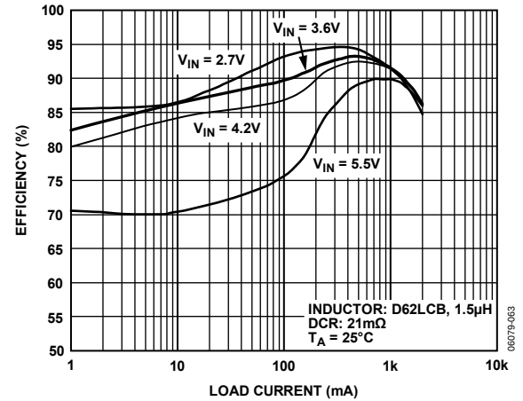
Figure 14. Efficiency—ADP2107 (1.8 V)
