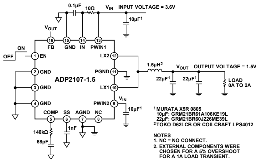
Figure 57. Application Circuit— V_{IN} = 3.6V , V_{OUT} = 1.5V , Load = 0A to 2A
