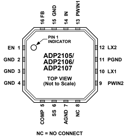
Figure 4. Pin Configuration
