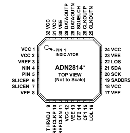
Figure 5. Pin Configuration
