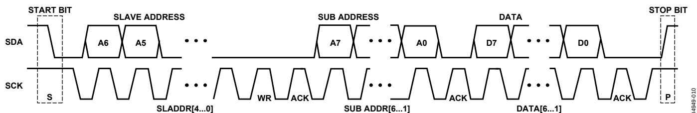
Figure 10. I 2 C Data Transfer Timing
