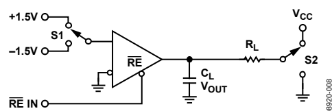
Figure 21. Receiver Enable/Disable
