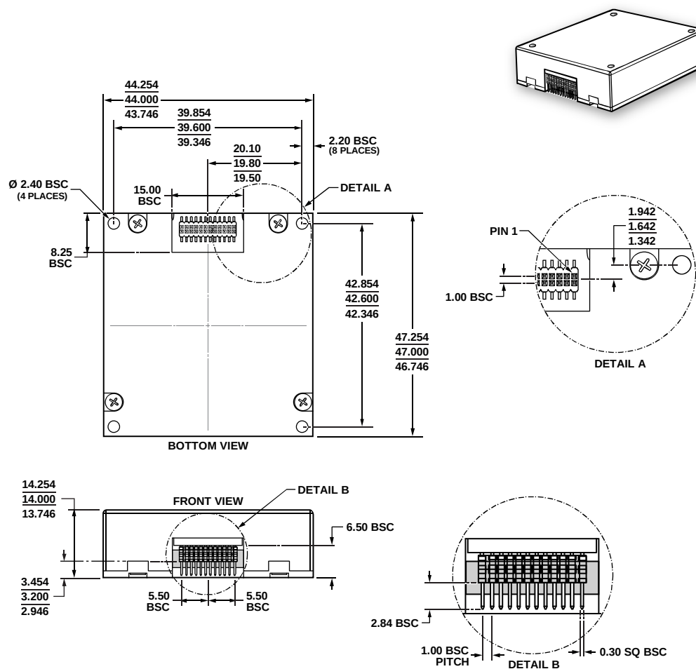
Figure 32. 24-Lead Module with Connector Interface [MODULE] (ML-24-6)
