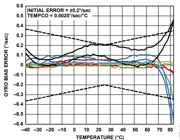
Figure 10. Gyroscope Bias Error and Hysteresis vs. Temperature
