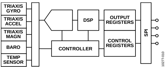
Figure 12. Basic Operation
