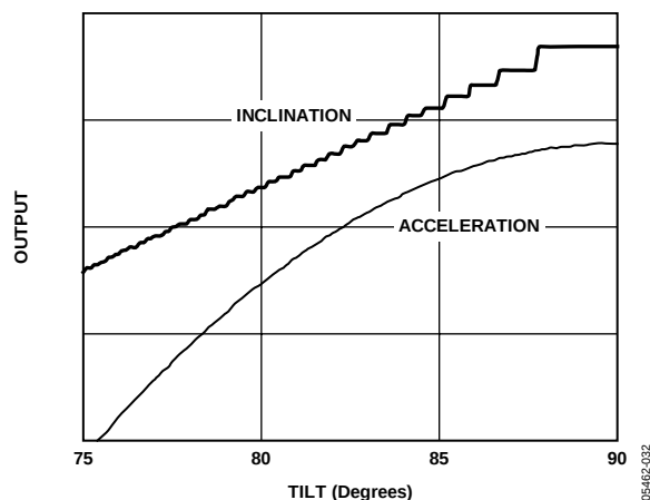
Figure 32. Acceleration and Inclination Angle vs. Actual Tilt Angle
