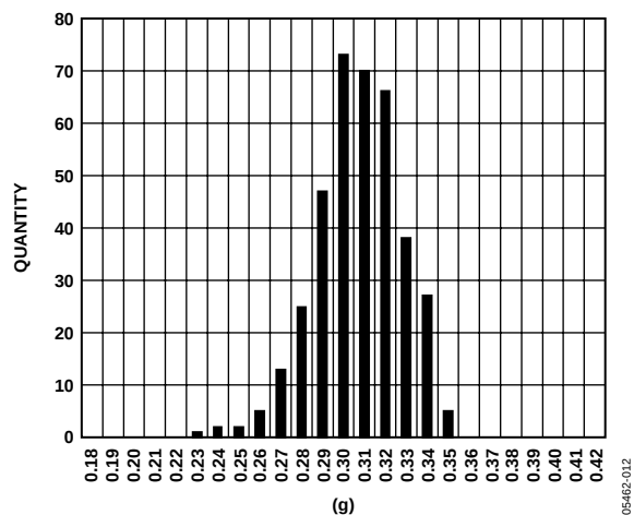
Figure 12. Y-Axis Self-Test Level at 25°C/3.3 V
