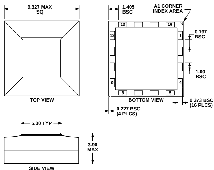
Figure 43. 16-Terminal Land Grid Array [LGA] (CC-16-2) Dimensions shown in millimeters
