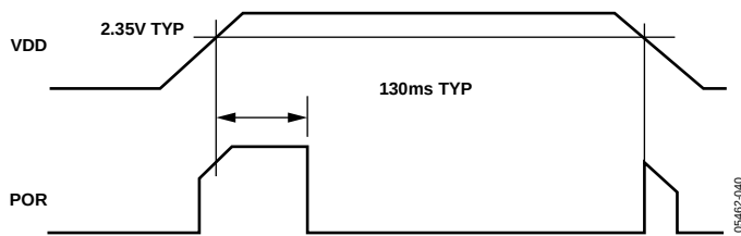
Figure 40. Internal Power-On Reset Operation
