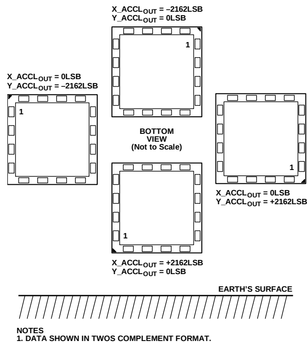
Figure 39. Output Response vs. Orientation
