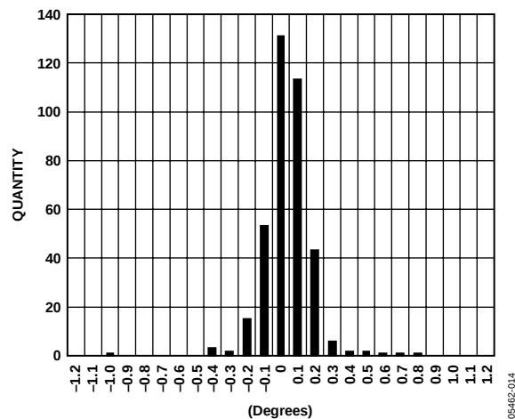
Figure 14. Inclination Offset Distribution at 25°C/3.3 V/0 g
