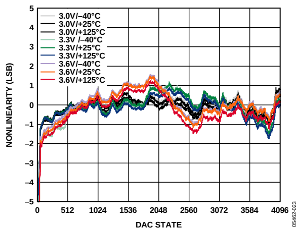
Figure 23. Typical DAC Integral Nonlinearity
