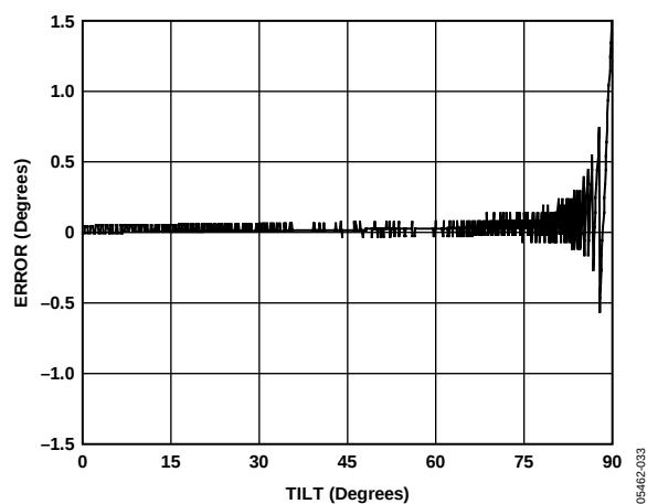
Figure 33. Inclusion Quantization Error
