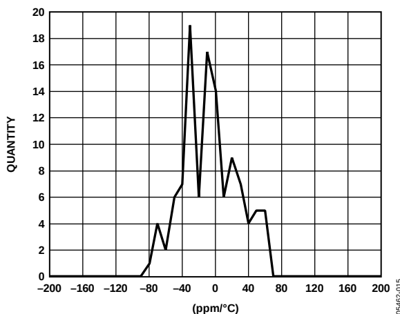
Figure 15. Inclination Offset Tempco Histogram at 3.3 V
