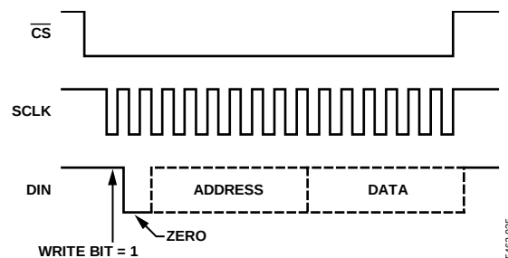
Figure 35. Control Register Write Command Sequence of SPI Signals
