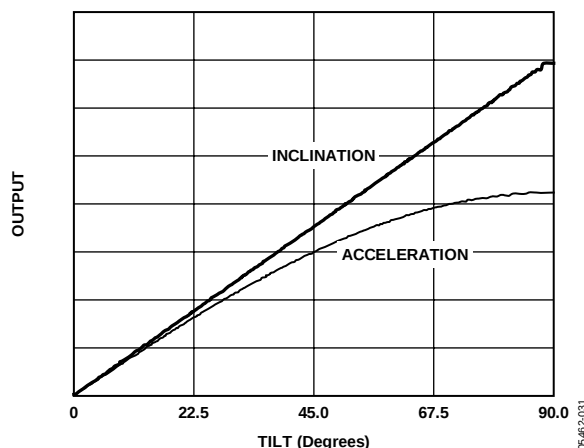
Figure 31. Acceleration and Inclination Angle vs. Actual Tilt Angle
