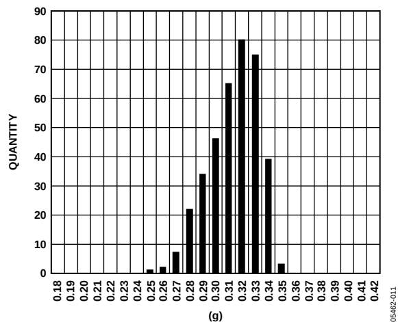
Figure 11. X-Axis Self-Test Level at 25°C/3.3 V
