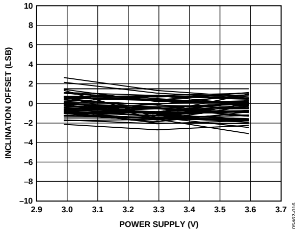
Figure 16. Inclination Offset vs. Supply at 25°C
