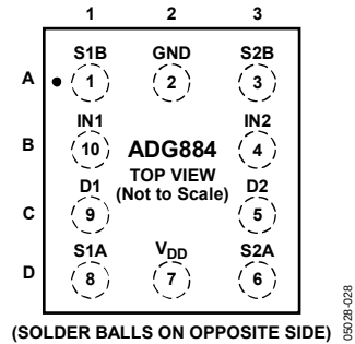
Figure 3. WLCSP Pin Configuration
