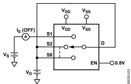
Figure 22. I_S (Off)
