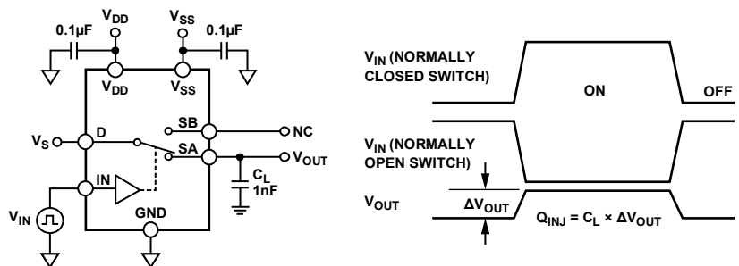
Figure 31. Charge Injection
