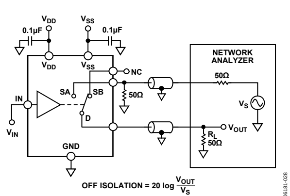
Figure 32. Off Isolation
