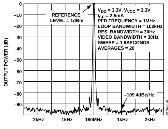
Figure 10. Close-In Phase Noise at 160 MHz (1 MHz Channel Spacing)
