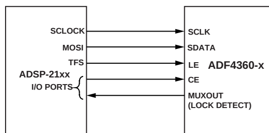
Figure 26. ADSP-21xx to ADF4360-x Interface
