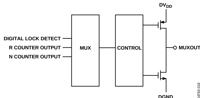
Figure 18. MUXOUT Circuit
