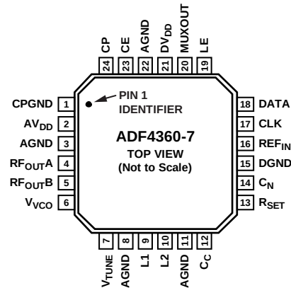
NOTES 1. THE EXPOSED PAD MUST BE CONNECTED TO AGND. Figure 3. Pin Configuration
