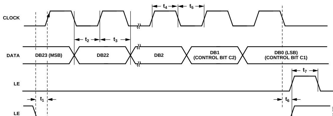
Figure 2. Timing Diagram
