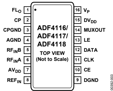
Figure 3. Pin Configuration
