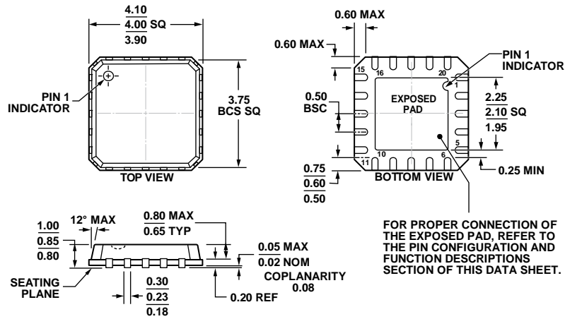
COMPLIANT TO JEDEC STANDARDS MO-220-VGGD-1 Figure 40. 20-Lead Lead Frame Chip Scale Package [LFCSQ_VQ] 4 mm × 4 mm Body, Very Thin Quad (CP-20-1) Dimensions shown in millimeters
