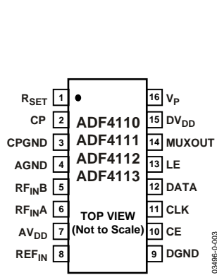
Figure 3. TSSOP Pin Configuration
