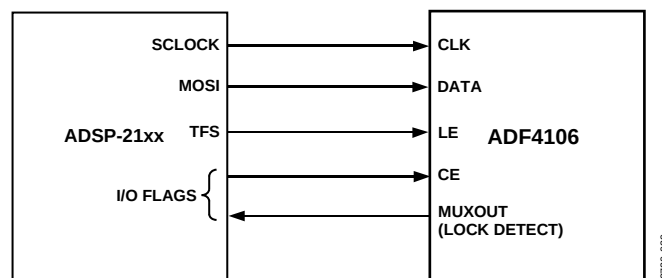
Figure 24. ADSP-21xx-to-ADF4106 Interface
