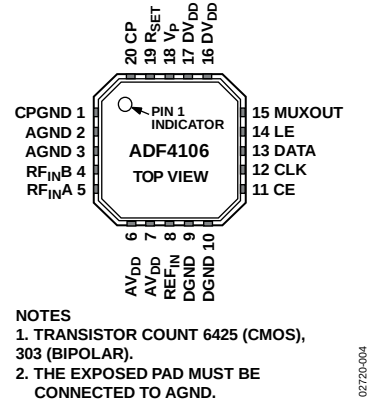
Figure 4. 20-Lead LFCSP_VQ Pin Configuration
