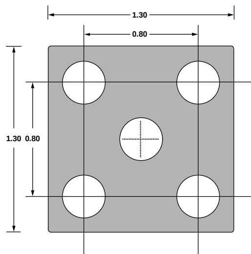
Figure 67. Recommended PCB Thermal Attach Pad Dimensions (mm)
