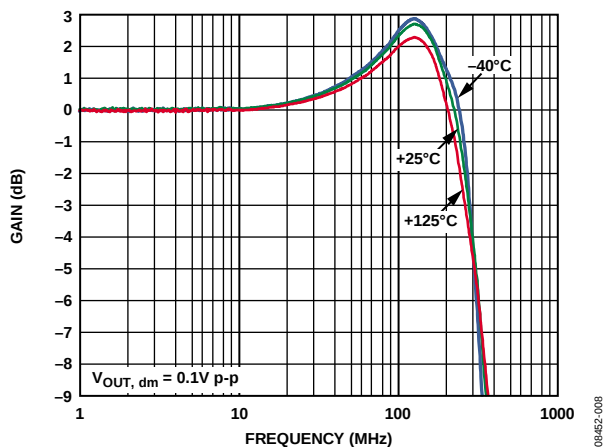
Figure 8. Small Signal Frequency Response for Various Temperatures
