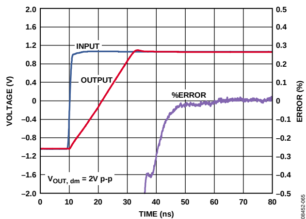
Figure 49. 0.1% Settling Time
