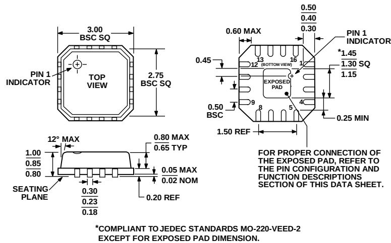
Figure 69. 16-Lead Lead Frame Chip Scale Package [LFCSP_VQ] 3 mm × 3 mm Body, Very Thin Quad (CP-16-2) Dimensions shown in millimeters
