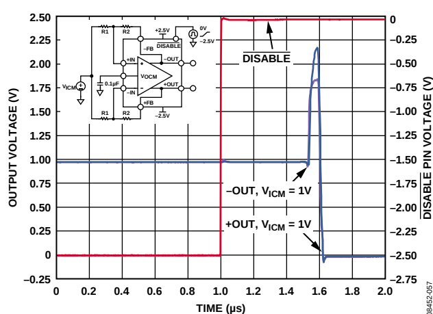
Figure 41. \overline{\text{DISABLE}} Pin Turn-On Time
