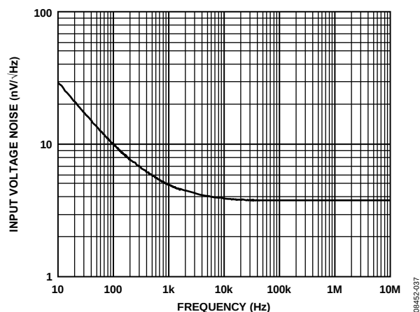
Figure 37. Voltage Noise Spectral Density, Referred to Input
