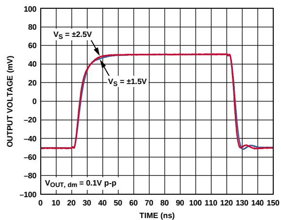
Figure 48. V_{OCM} Small Signal Transient Response
