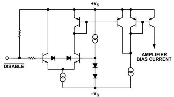
Figure 62. \overline{\text{DISABLE}} Pin Circuit
