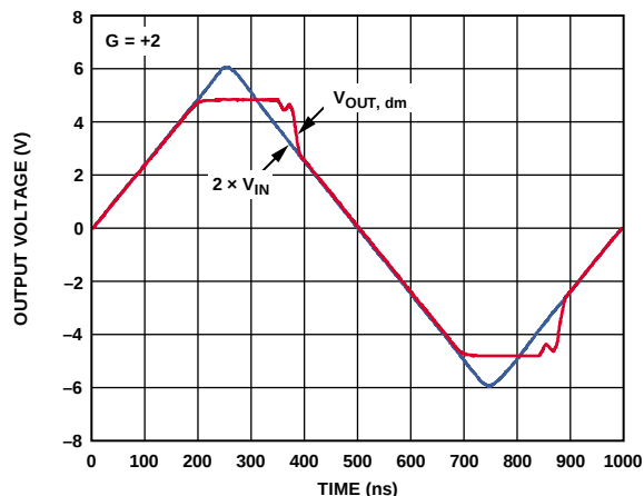
Figure 36. Output Overdrive Recovery, G = 2
