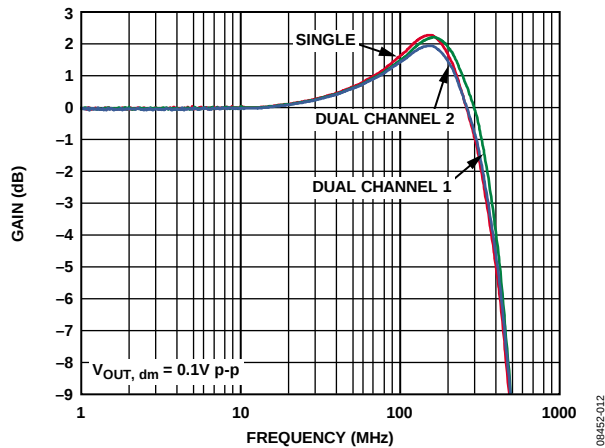
Figure 12. Small Signal Frequency Response for Various Packages
