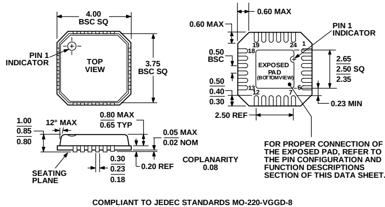
Figure 70. 24-Lead Lead Frame Chip Scale Package [LFCSP_VQ] 4 mm × 4 mm Body, Very Thin Quad (CP-24-3) Dimensions shown in millimeters
