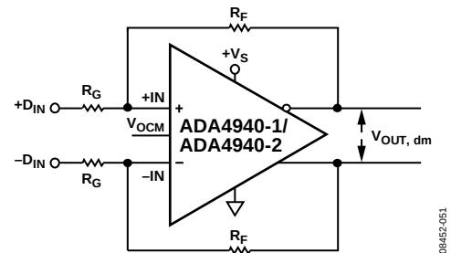
Figure 56. ADA4940-1/ADA4940-2 Configured for Balanced (Differential) Inputs
