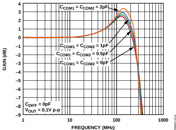
Figure 14. Small Signal Frequency Response for Various Capacitive Loads
