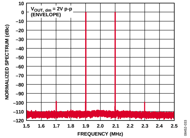
Figure 33. 2 MHz Intermodulation Distortion
