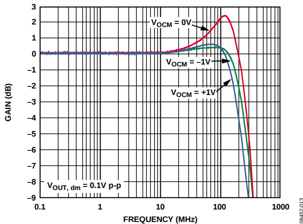
Figure 13. Small Signal Frequency Response at Various V_{OCM} Levels
