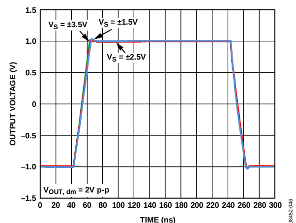
Figure 46. Large Signal Transient Response for Various Supplies
