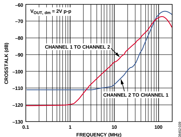
Figure 39. Crosstalk vs. Frequency, ADA4940-2
