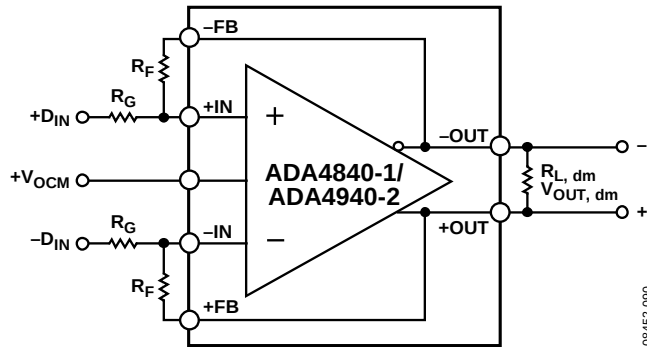
Figure 53. Circuit Definitions
