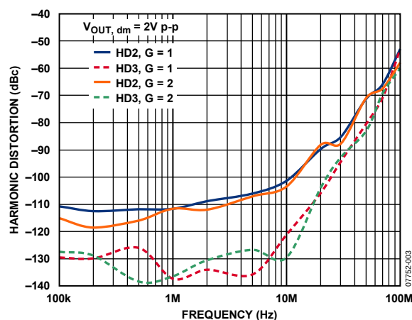
Figure 3. Harmonic Distortion vs. Frequency at Various Gains
