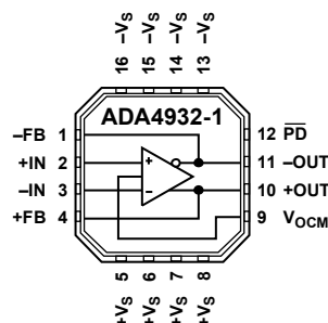
Figure 1. ADA4932-1
