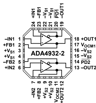
Figure 2. ADA4932-2
