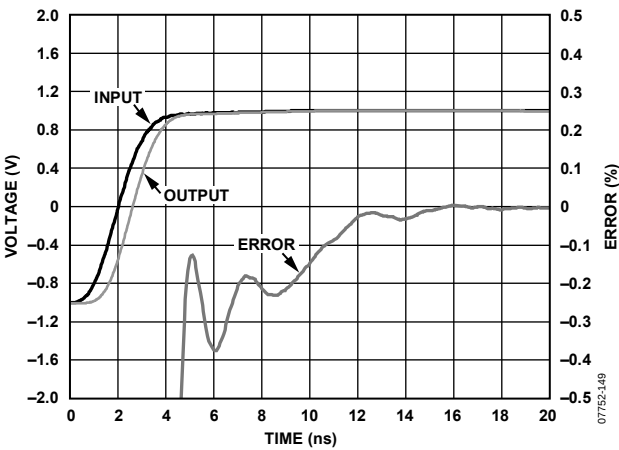
Figure 49. Settling Time
