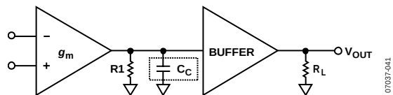
Figure 44. Topology
