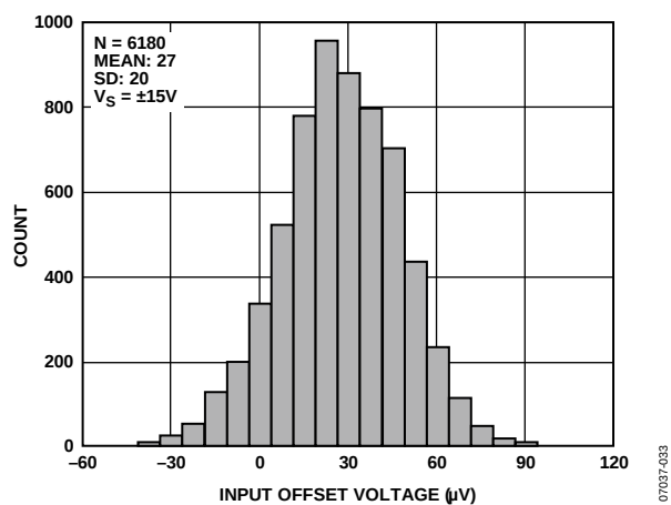
Figure 37. Input Offset Voltage Distribution, V_S = \pm 15\text{ V}
