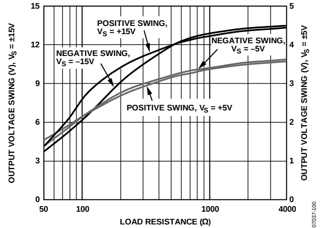
Figure 34 Output Swing vs. Load, G = +2 , \text{Load} = R_L // (R_F + R_G)
