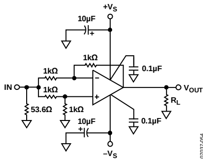
Figure 40. Common-Mode Rejection
