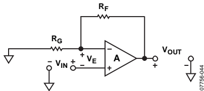
Figure 41. Noninverting Configuration
