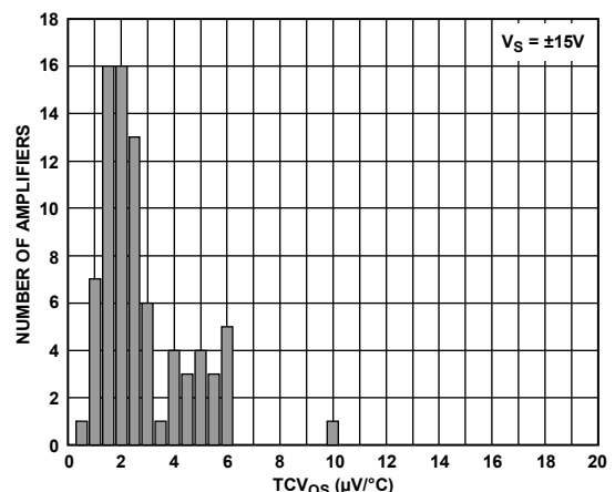
Figure 8. Offset Voltage Drift Distribution, V_S = \pm 15 V
