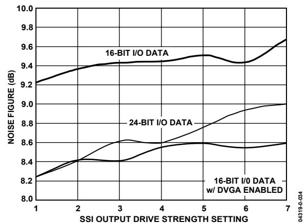
Figure 34. NF vs. SSI Output Drive Strength ( V_{DDX} = 3.0\text{ V} , F_{CLK} = 18\text{ MSPS} , BW = 10\text{ kHz} )
