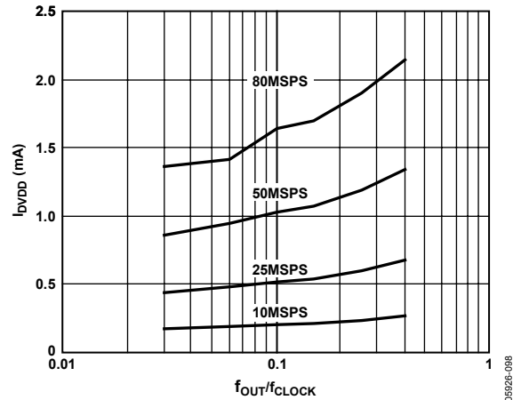
Figure 85. I_{DVDD} vs. f_{OUT}/f_{CLOCK} Ratio @ DVDD = 1.8 V
