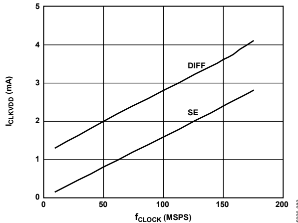
Figure 86. I_{CLKVDD} vs. f_{CLOCK} @ CLKVDD = 3.3 V
