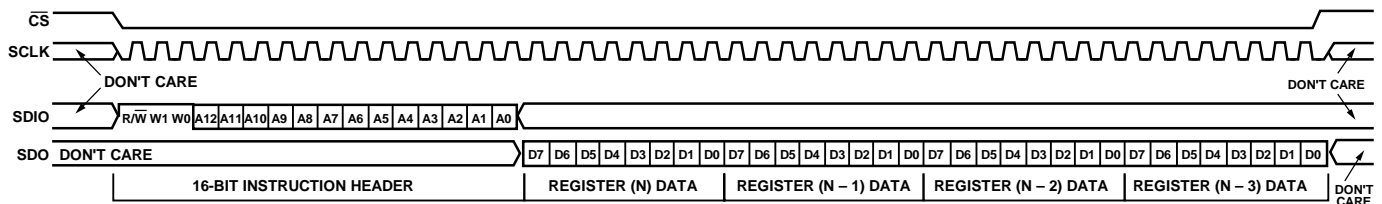
Figure 55. Serial Control Port Read—MSB First, 16-Bit Instruction, Four Bytes of Data
