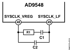
Figure 47. External Loop Filter Schematic
