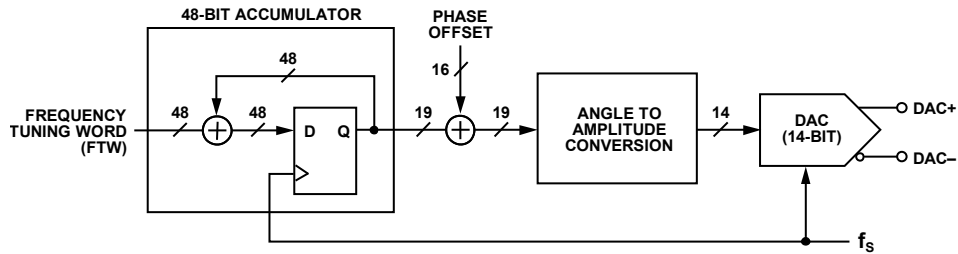
Figure 43. DDS Block Diagram
