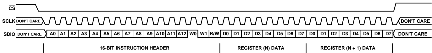
Figure 59. Serial Control Port Write—LSB First, 16-Bit Instruction, Two Bytes of Data
