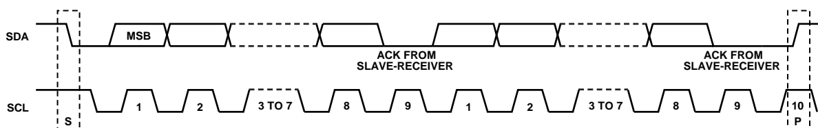
Figure 63. Acknowledge Bit
