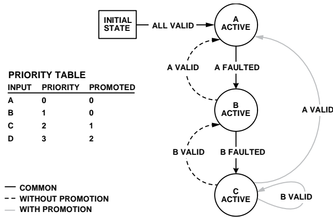
Figure 36. Example of Priority Promotion
