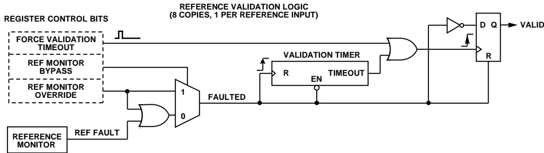
Figure 35. Reference Validation Override
