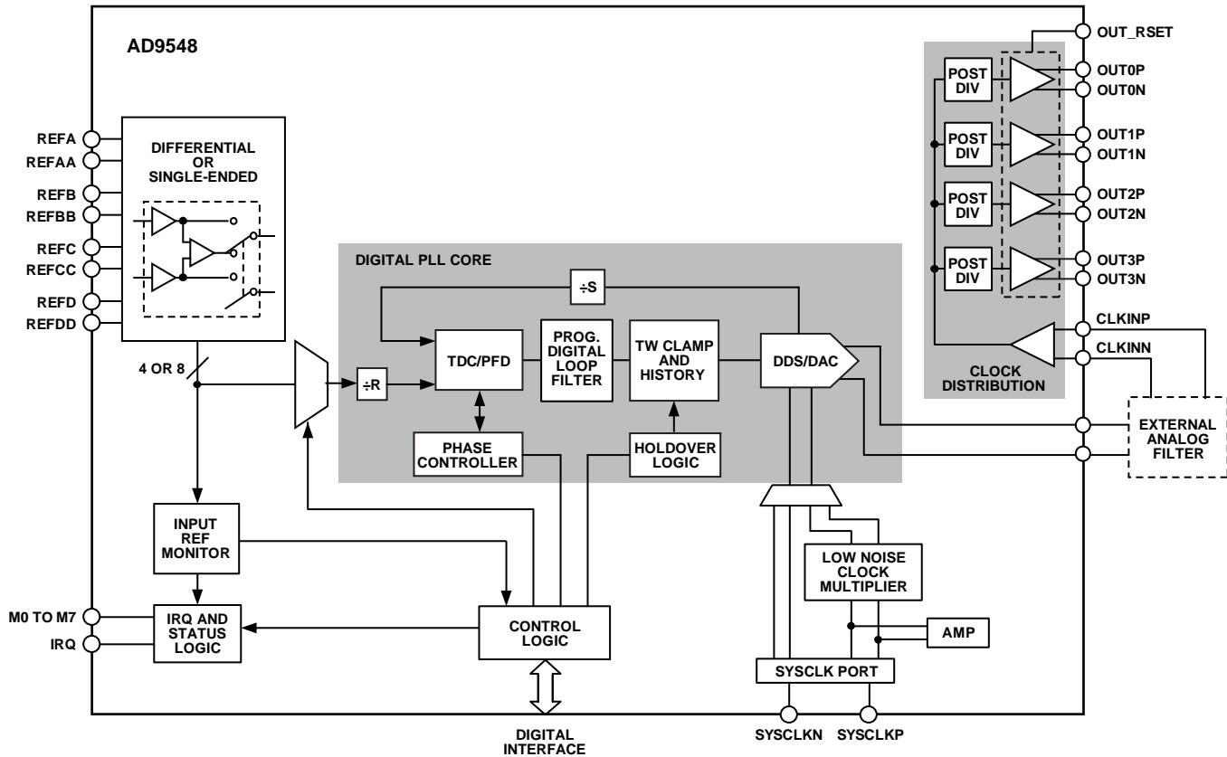
Figure 34. Detailed Block Diagram
