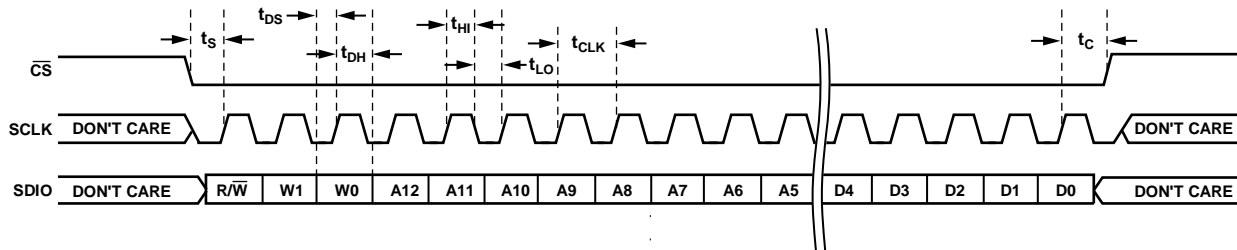
Figure 57. Serial Control Port Write—MSB First, 16-Bit Instruction, Timing Measurements
