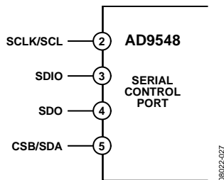
Figure 53. Serial Control Port
