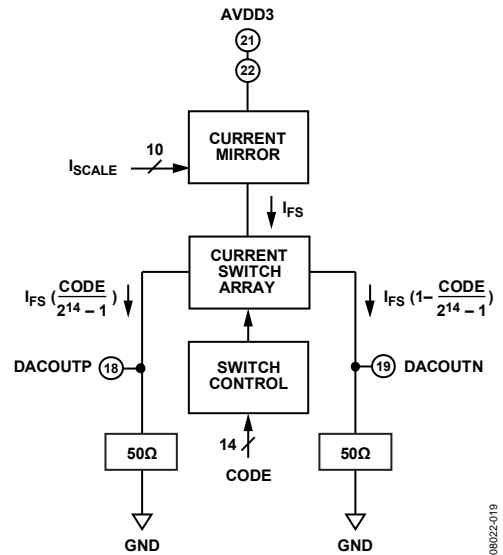
Figure 44. DAC Output Pins
