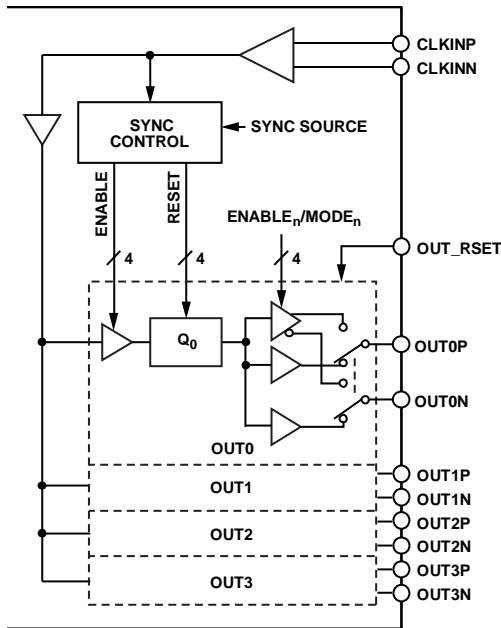
Figure 48. Clock Distribution
