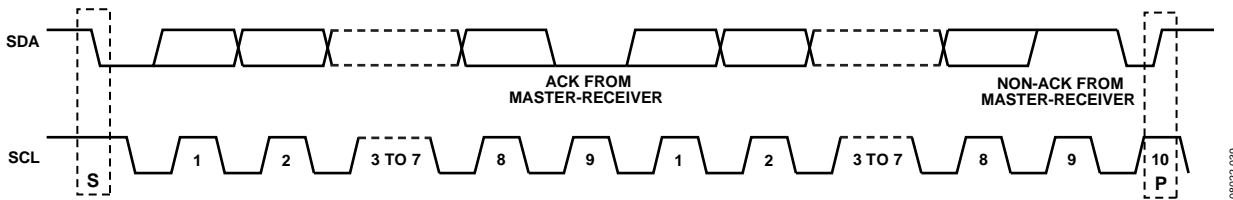
Figure 65. Data Transfer Process (Master Read Mode, 2-Byte Transfer)
