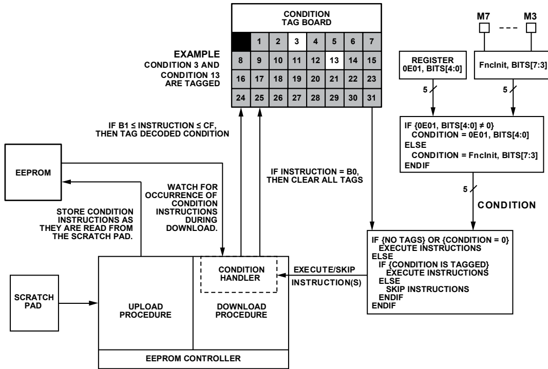
Figure 51. EEPROM Conditional Processing
