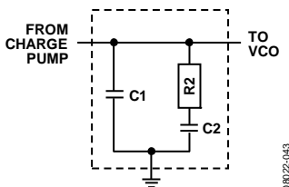
Figure 69. Second Order Analog Loop Filter
