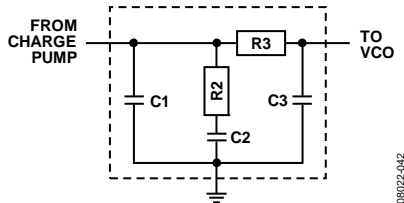
Figure 68. Third Order Analog Loop Filter
