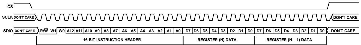
Figure 54. Serial Control Port Write—MSB First, 16-Bit Instruction, Two Bytes of Data
