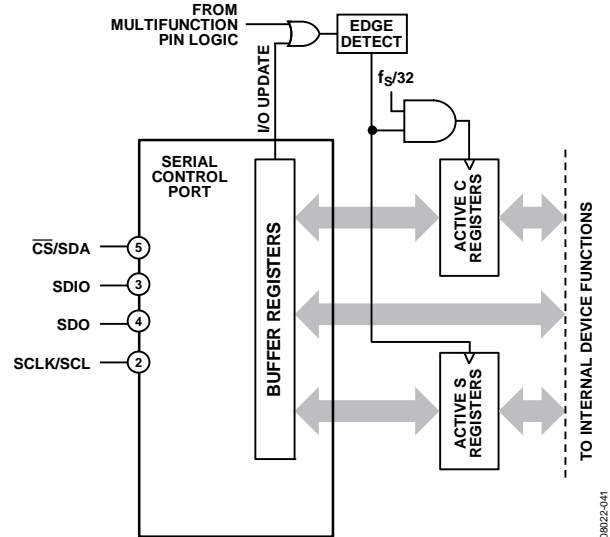
Figure 67. Buffered and Active Registers
