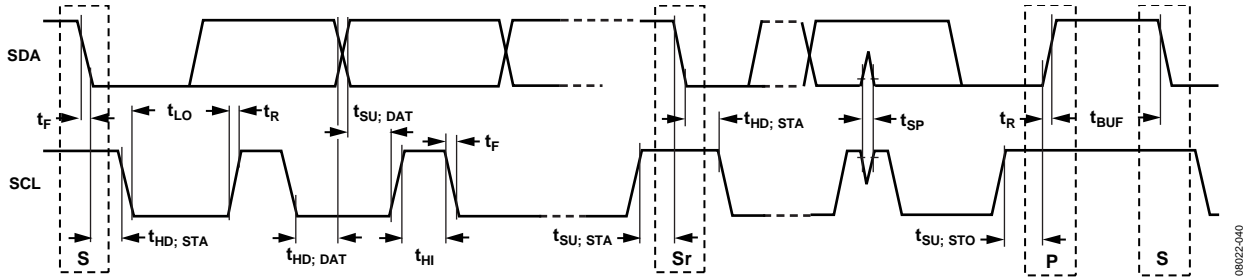
Figure 66. I 2 C Serial Port Timing
