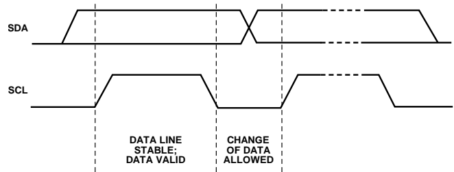
Figure 61. Valid Bit Transfer
