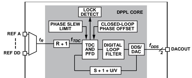
Figure 38. Digital PLL Core
