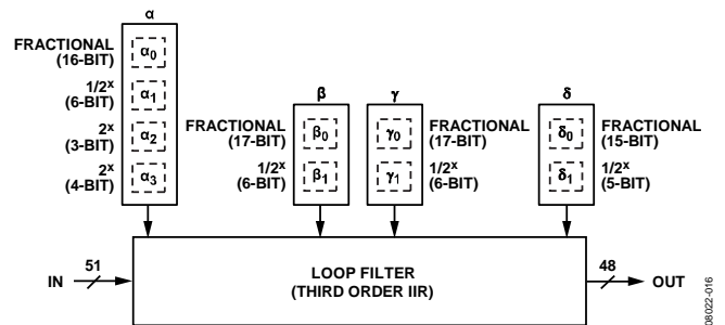
Figure 41. Third Order Digital IIR Loop Filter
