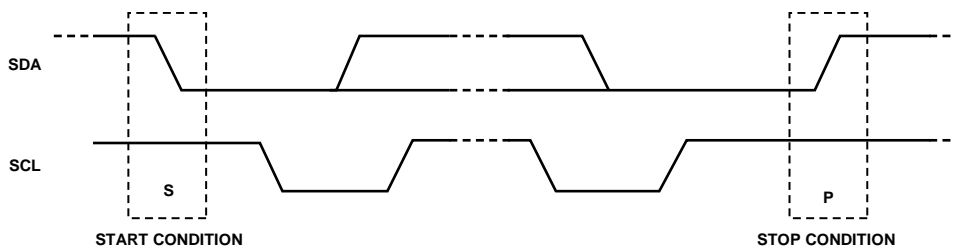
Figure 62. Start and Stop Conditions
