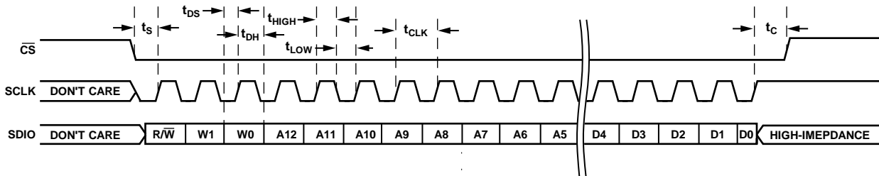
Figure 56. Serial Control Port Read—MSB First, 16-Bit Instruction, One Byte of Data
