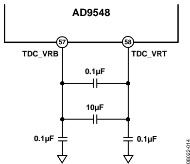
Figure 39. TDC Pin Connections
