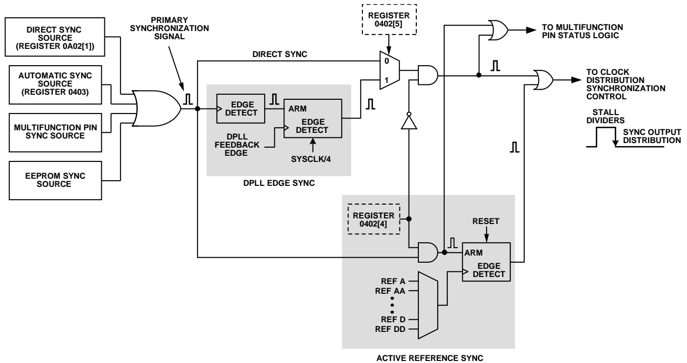
Figure 49. Output Synchronization Block Diagram
