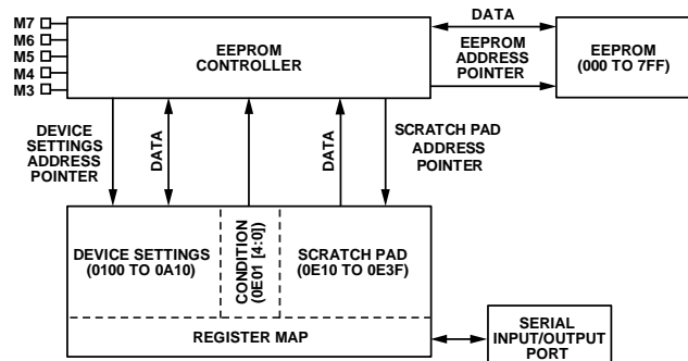
Figure 50. EEPROM Functional Diagram
