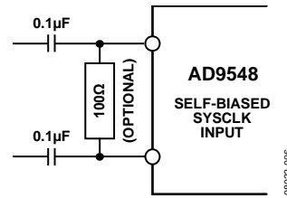
Figure 31. SYSCLKx Input
