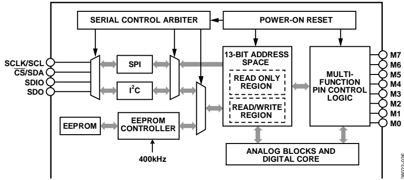
Figure 52. Serial Port Functional Diagram
