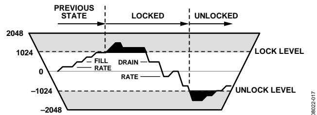
Figure 42. Lock Detector Diagram
