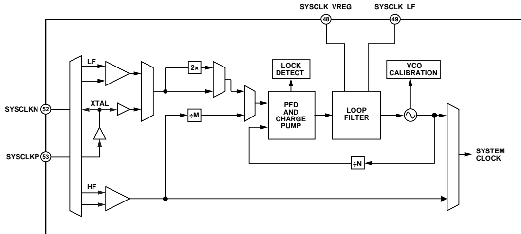
Figure 46. System Clock Block Diagram
