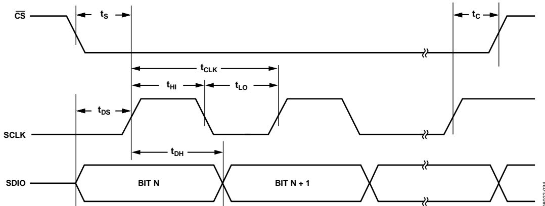
Figure 60. Serial Control Port Timing—Write
