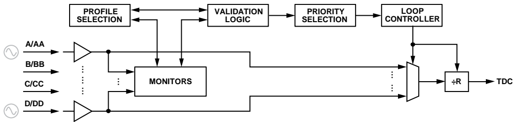
Figure 37. Reference Clock Block Diagram
