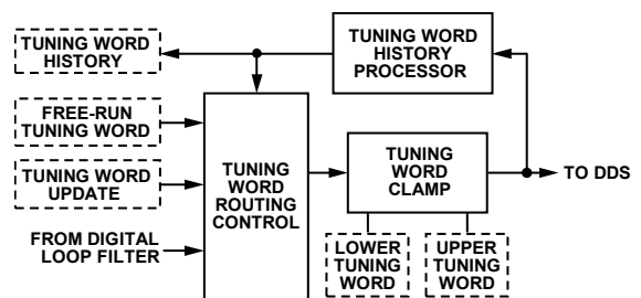
Figure 45. Tuning Word Processing
