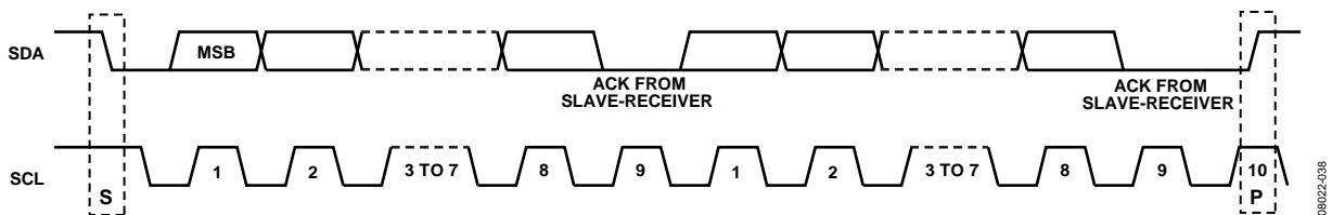
Figure 64. Data Transfer Process (Master Write Mode, 2-Byte Transfer)
