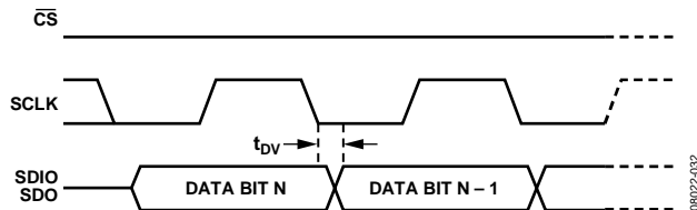
Figure 58. Timing Diagram for Serial Control Port Register Read
