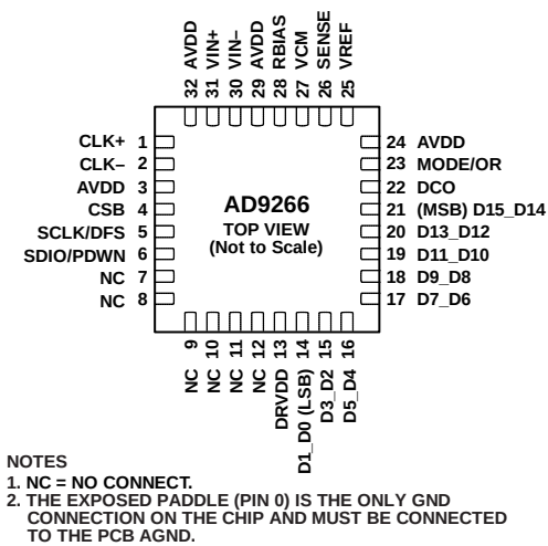
Figure 3. Pin Configuration
