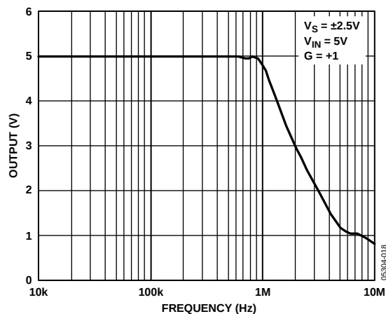
Figure 26. Maximum Output Swing vs. Frequency
