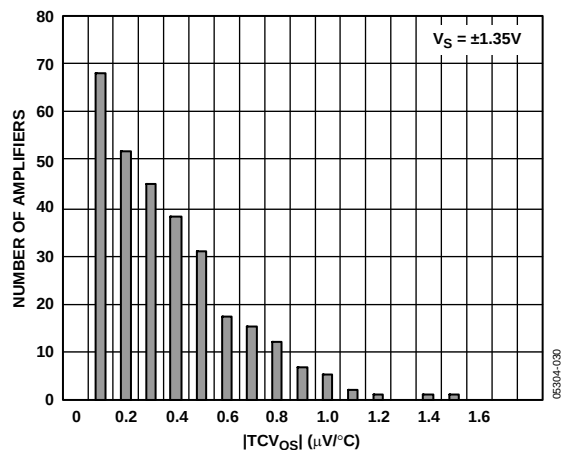
Figure 35. |TCV_{OS}| Distribution
