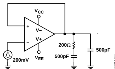
Figure 57. Snubber Network
