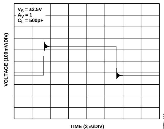
Figure 56. Driving Heavy Capacitive Loads Without Compensation
