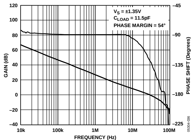
Figure 50. Open-Loop Gain and Phase vs. Frequency
