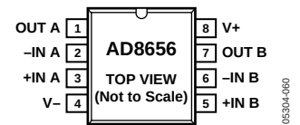
Figure 4. AD8656 8-Lead SOIC (R-8)
