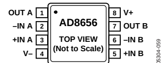
Figure 2. AD8656 8-Lead MSOP (RM-8)
