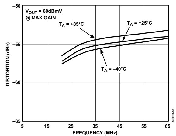
Figure 11. Third-Order Harmonic Distortion vs. Frequency vs. Temperature
