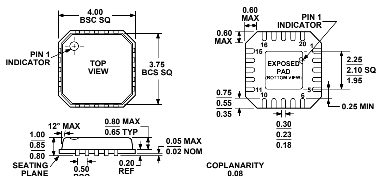
Figure 33. 20-Lead Frame Chip Scale Package [LFCS_P_VQ] 4 mm x 4 mm Body, Very Thin Quad (CP-20-1) Dimensions shown in millimeters
