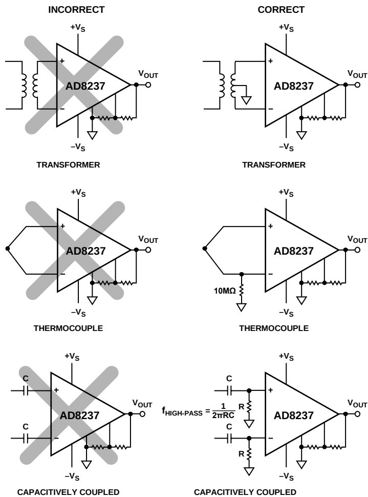
Figure 74. Creating an I_{BIAS} Path
