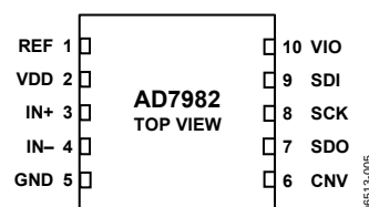
Figure 5. 10-Lead QFN (LFCSP) Pin Configuration
