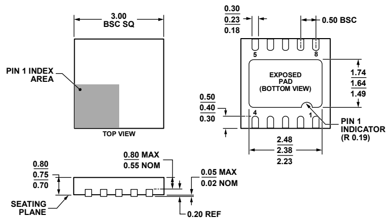
Figure 44. 10-Lead Lead Frame Chip Scale Package [QFN (LFCSP_WD)] 3 mm × 3 mm Body, Very Very Thin, Dual Lead (CP-10-9)
