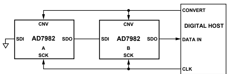
Figure 37. Chain Mode Without Busy Indicator Connection Diagram
