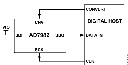
Figure 29. \overline{\text{CS}} Mode, 3-Wire Without Busy Indicator Connection Diagram (SDI High)
