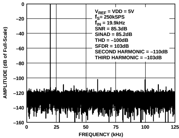
Figure 7. 20 kHz FFT, V_{REF} = V_{DD} = 5\text{ V}
