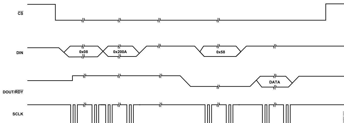
Figure 16. Single Conversion
