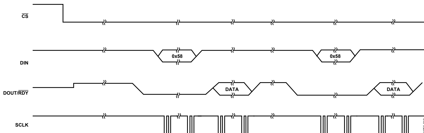
Figure 17. Continuous Conversion
