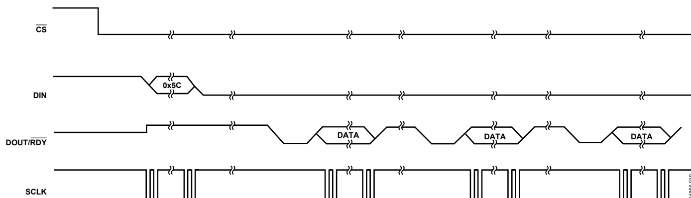
Figure 18. Continuous Read
