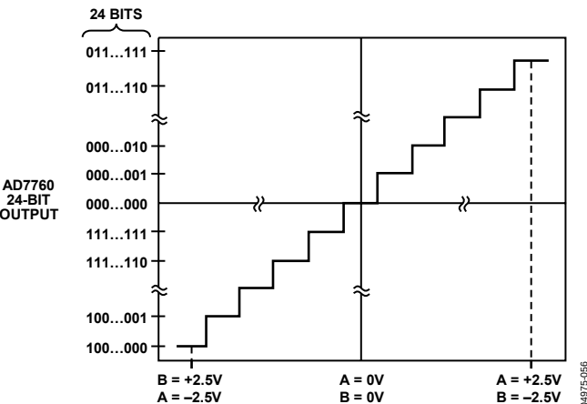
Figure 51. Transfer Function for the AD7760 Filtered Output Where V_A and V_B are Inputs to the On-Board Differential Amplifier A1
