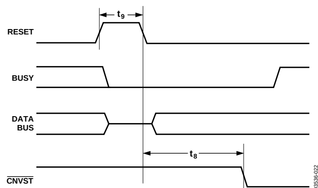
Figure 22. Reset Timing
