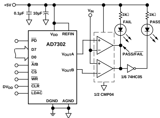
Figure 34. Programmable Window Detector
