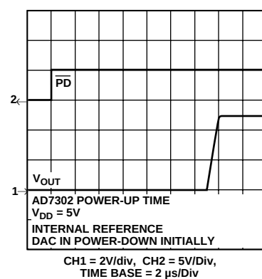
Figure 10. Exiting Power-Down (Full Power-Down)
